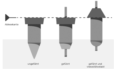
Fig. 4: Types of floats
