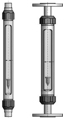
Fig. 2: Tubux M30 with female thread and flange connection
